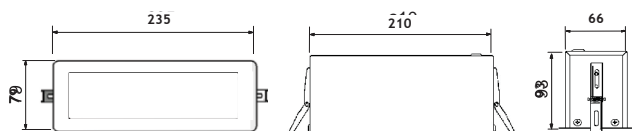
Vista Frontal
